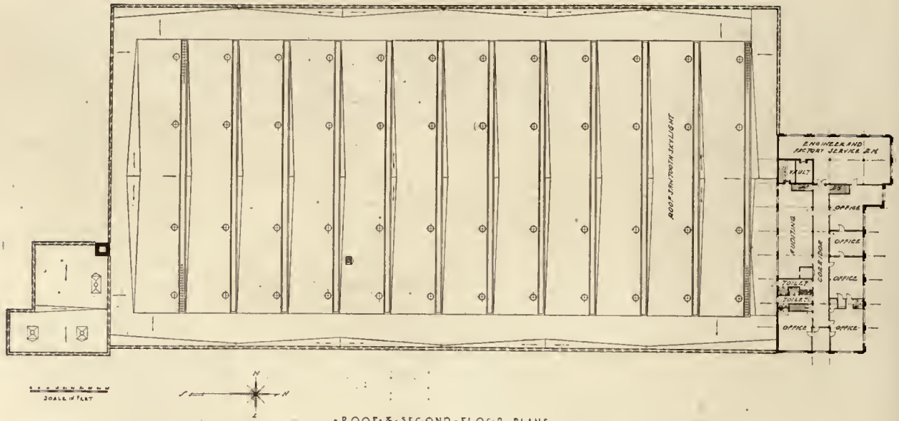
- ROOF & SECOND-FLOOR PLANS - BUILDING FOR WALKER VEHICLE CO., CHICAGO, ILL.
